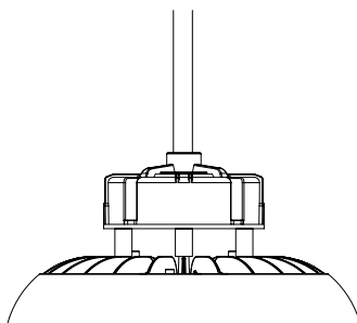
Pendant Mounting 3/4"
