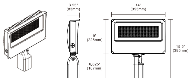
FLWA-150A with Slip Fitter
