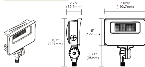
FLWA-30A with Knuckle
