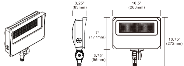
FLWA-90A with Knuckle
