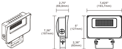
FLWA-30A with Trunnion
