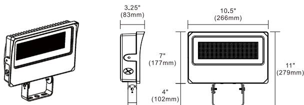
FLWA-90A with Trunnion
