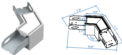
ILA-L120WDIDC-8AK
