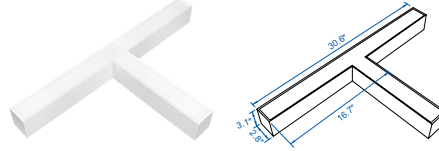
ILA-TDIDC(40)-8AK
