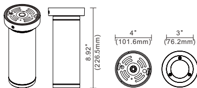
Ceilin Mount
